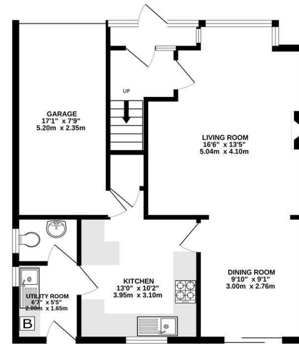
GROUND FLOOR 659 sq.ft. (61.2 sq.m.) approx.
